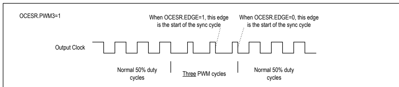
Figure 7-8. Embedded Sync in Output Clocks, Three PWM Cycles
